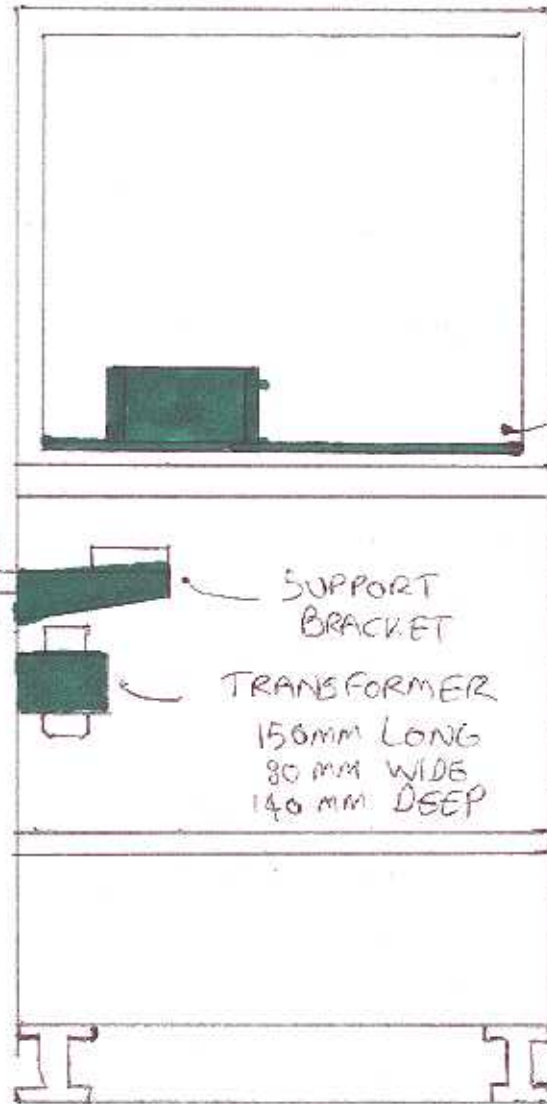
SIDE
