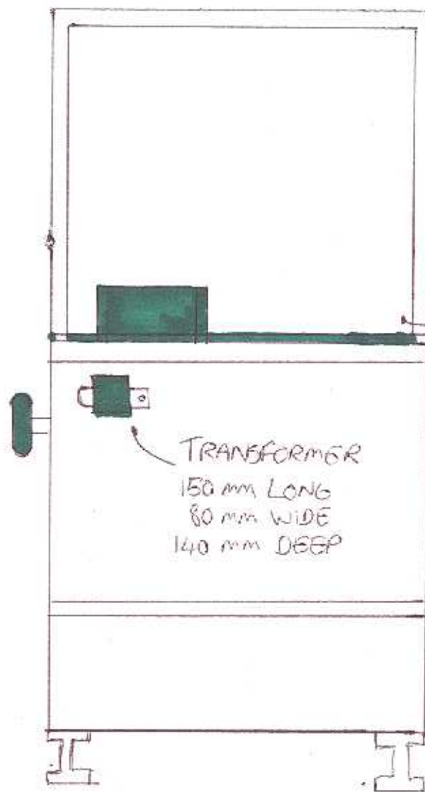
SIDE
