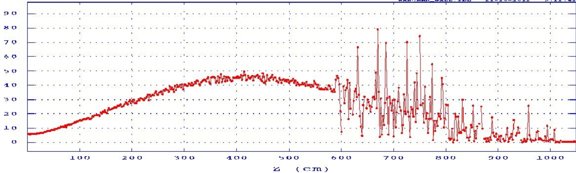
Magnetic field data from file: WANGNMR_WALL.DAT Problem title line is NMR Spectrometer Solenoid Magnet at Wang, NMR: Proposed Wall WANGNMR_WALL.TEL 11-25-2012 5:11:42
