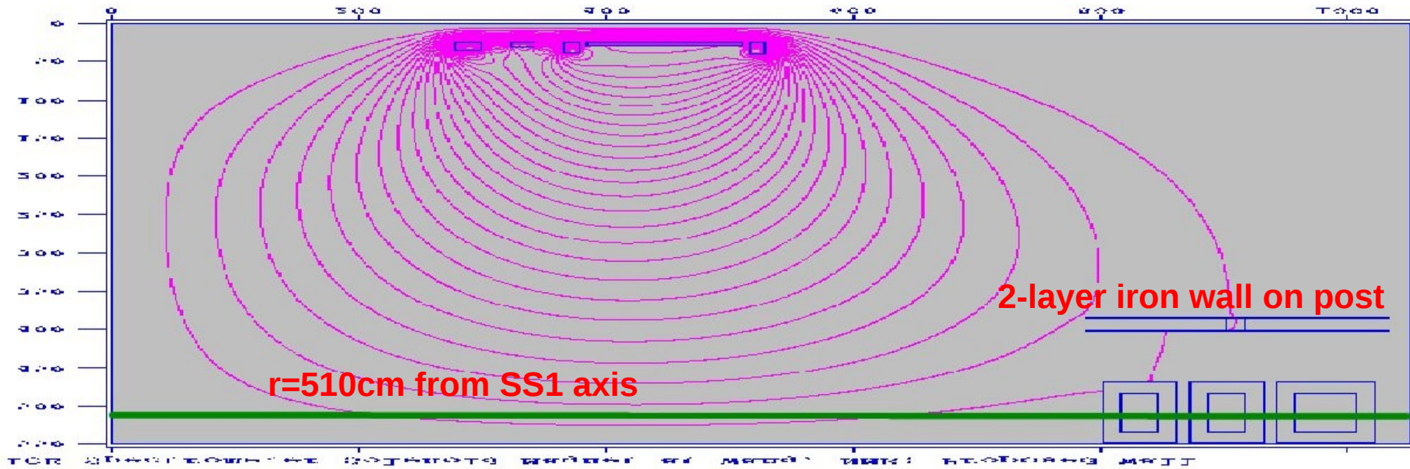
Magnetic field data from file: WANGNMR_WALL.DAT Problem title line is NMR Spectrometer Solenoid Magnet at Wang, NMR: Proposed Wall WANGNMR_WALL.TEL 11-25-2012 5:11:42
